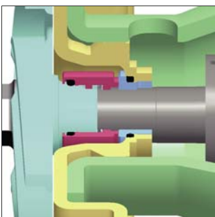
Single mechanical seal (standard)
