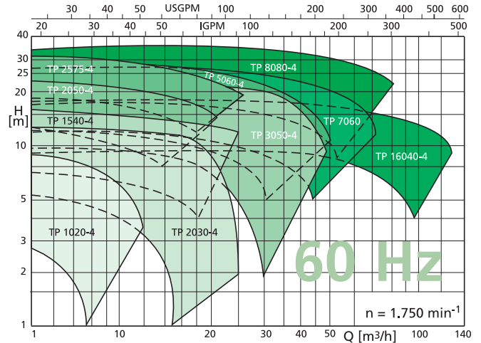
Pump performance curves type TP, n = 1.750 \text{ min}^{-1}
