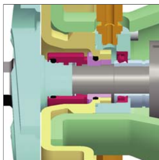
Single mechanical seal, flushed (quench)
