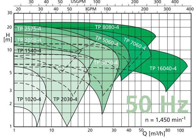
Pump performance curves type TP, n = 1.450 \text{ min}^{-1}
